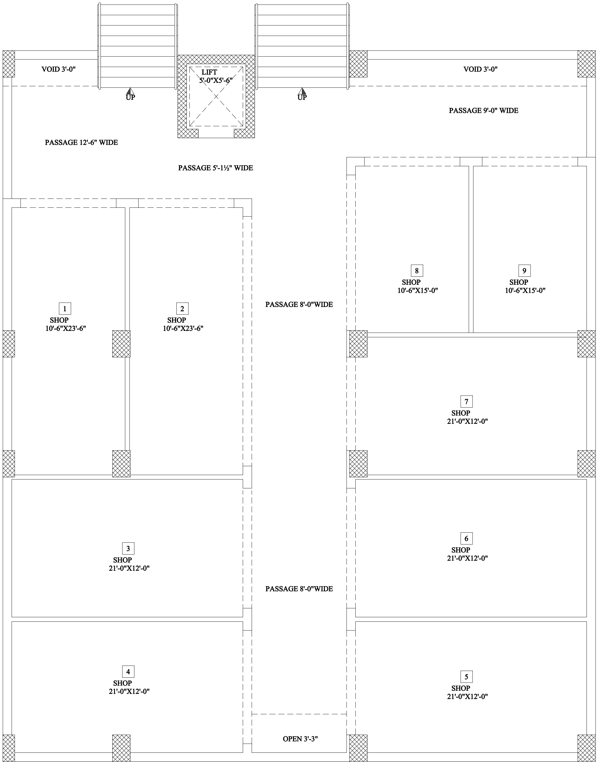
BASEMENT FLOOR PLAN COVERED AREA = 3000.00 Sq.ft.
