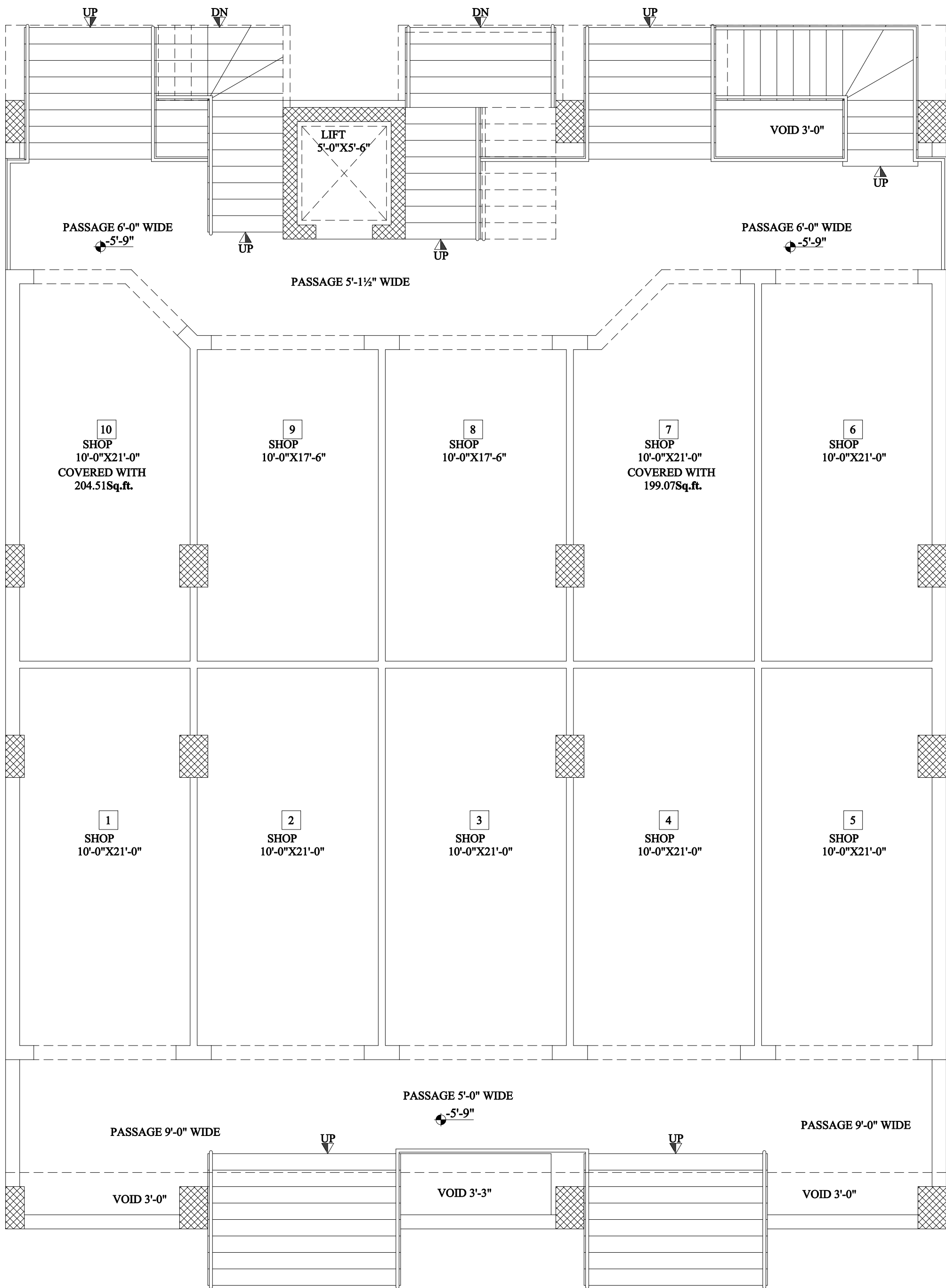
LOWER GROUND FLOOR PLAN COVERED AREA = 3000.00 Sq.ft.
