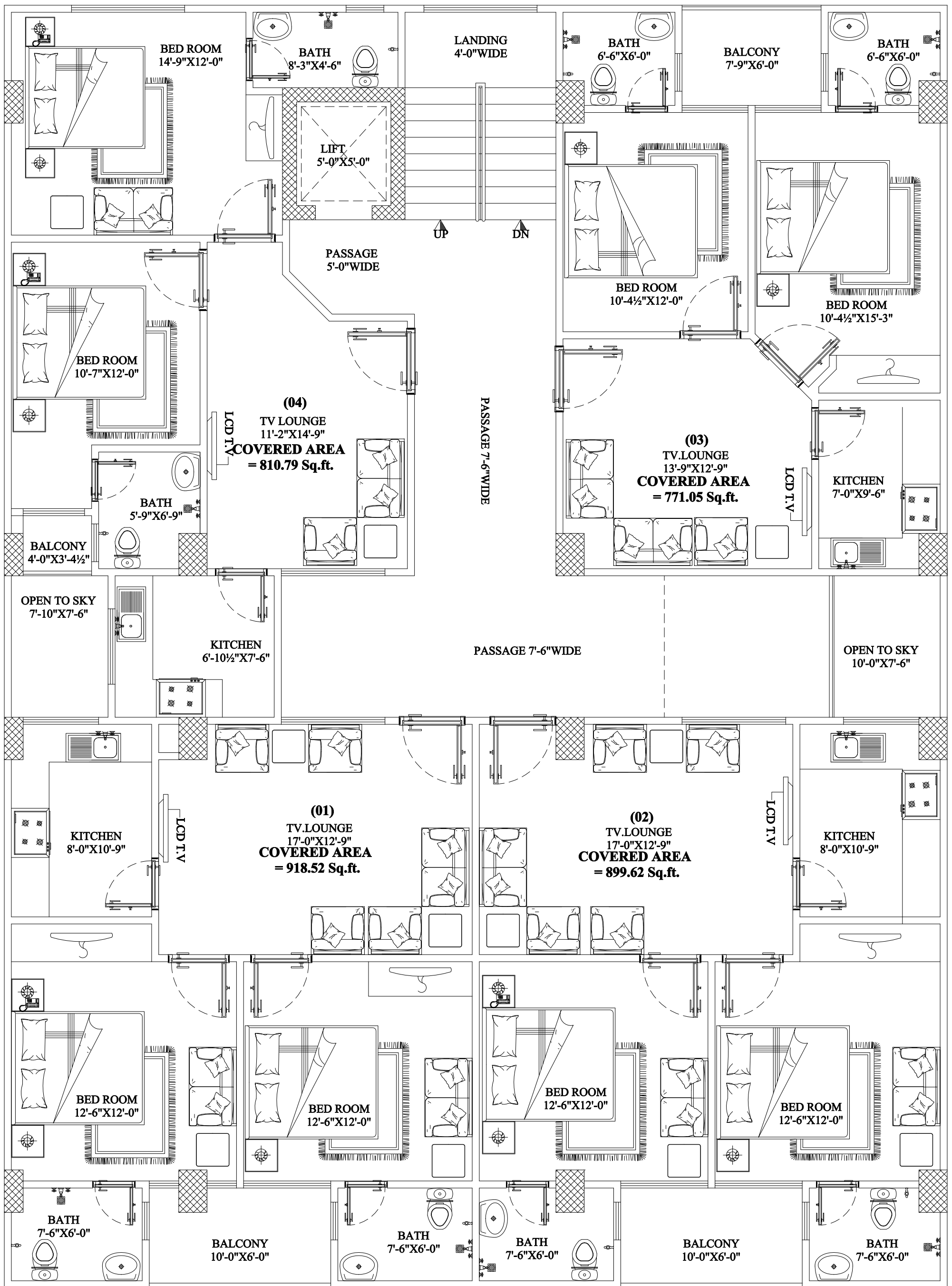
2nd To 5th FLOOR PLAN
